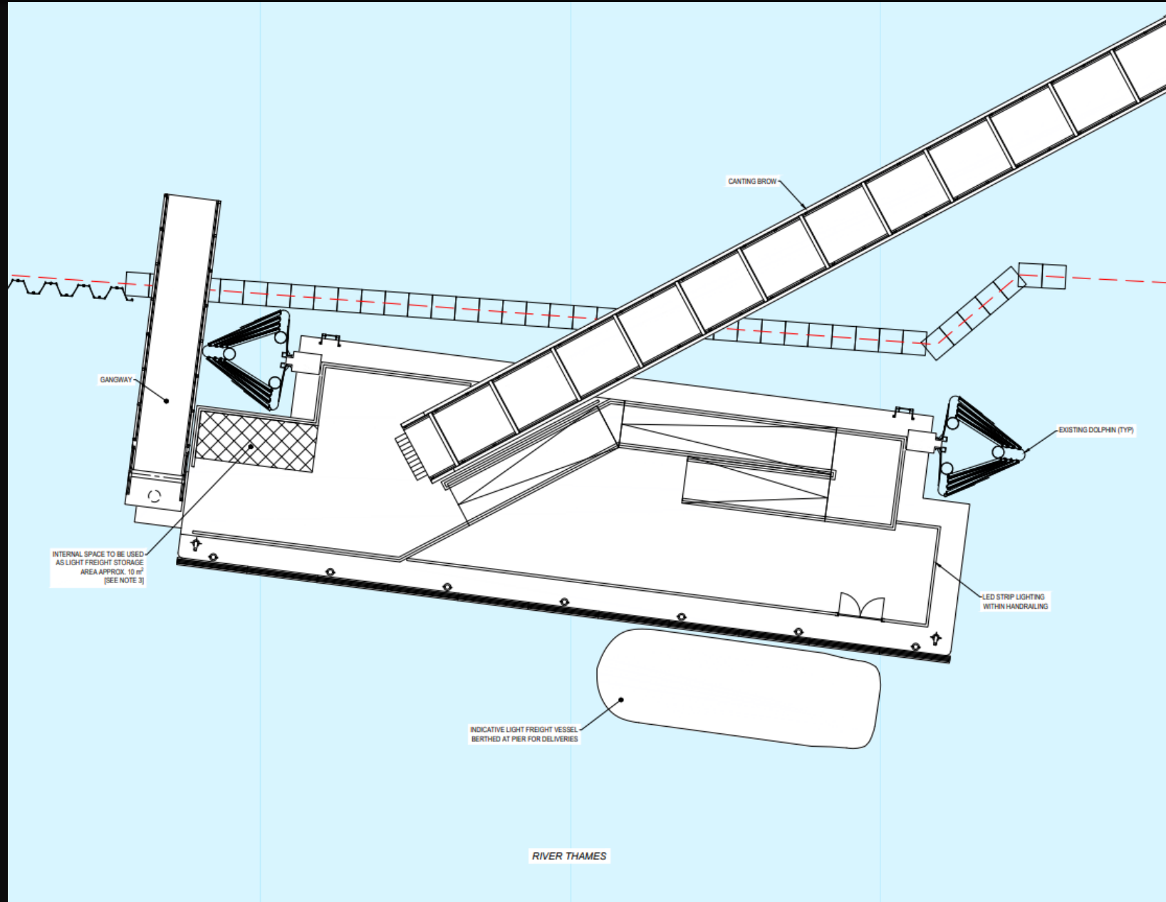
Proposed pier arrangement
