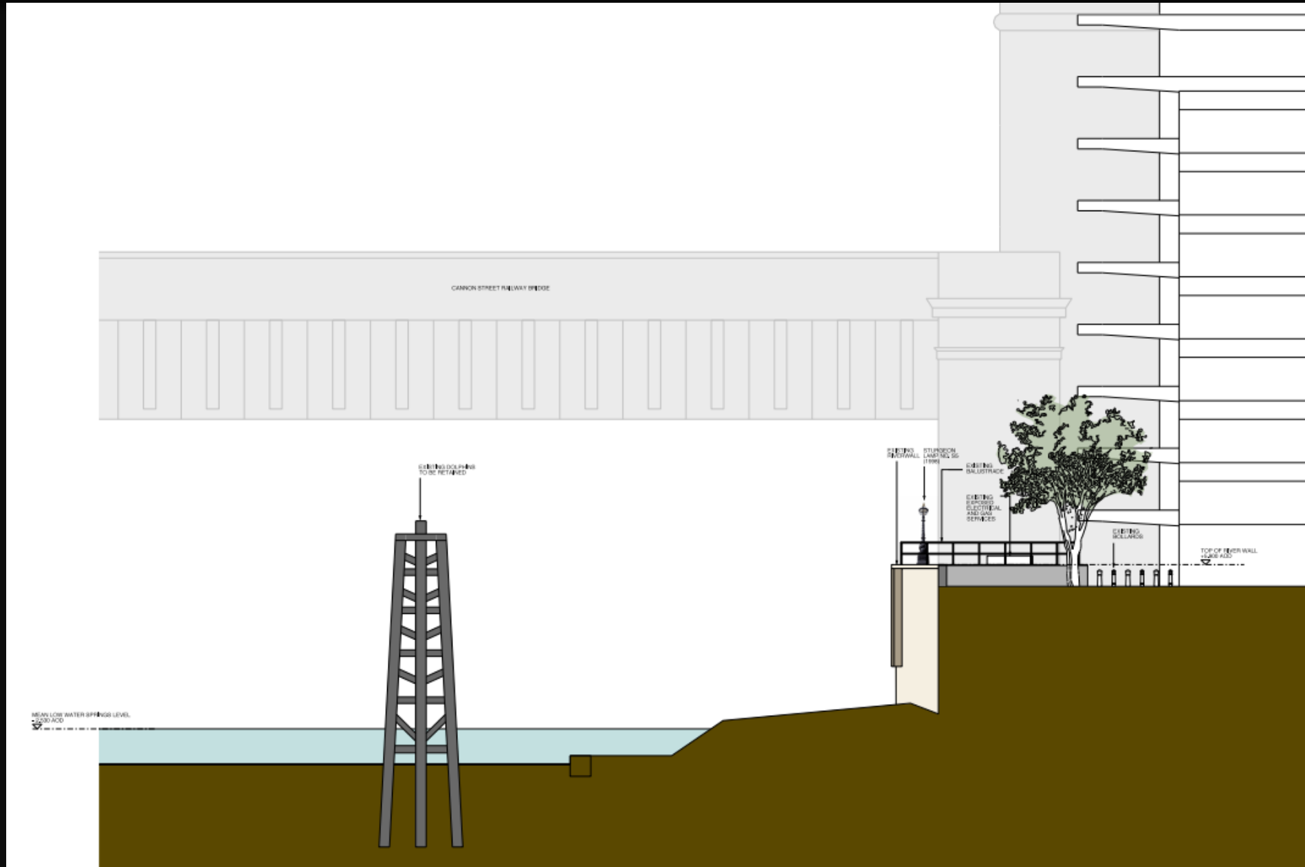
Existing Cross Section – Low Tide
